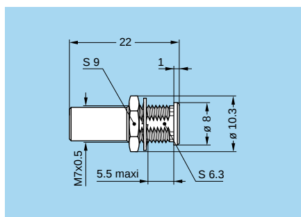
RAD Fixed coupler, nut fixing
