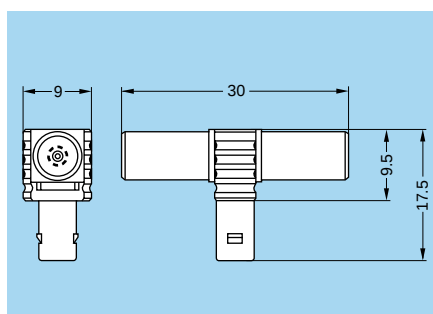
FTA T-plug with two sockets in line
