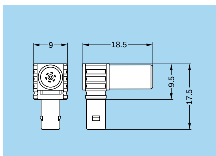
FTR Elbow plug (90°) with socket
