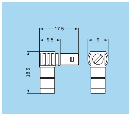
FLR Elbow plug (90°) with resistor
